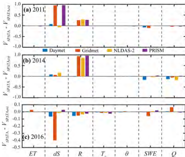
Figure 14. The difference between the predicted and actual changes from combined variability in P and T_{air} for WY2011 (a), WY2014 (b), and WY2016 (c).
