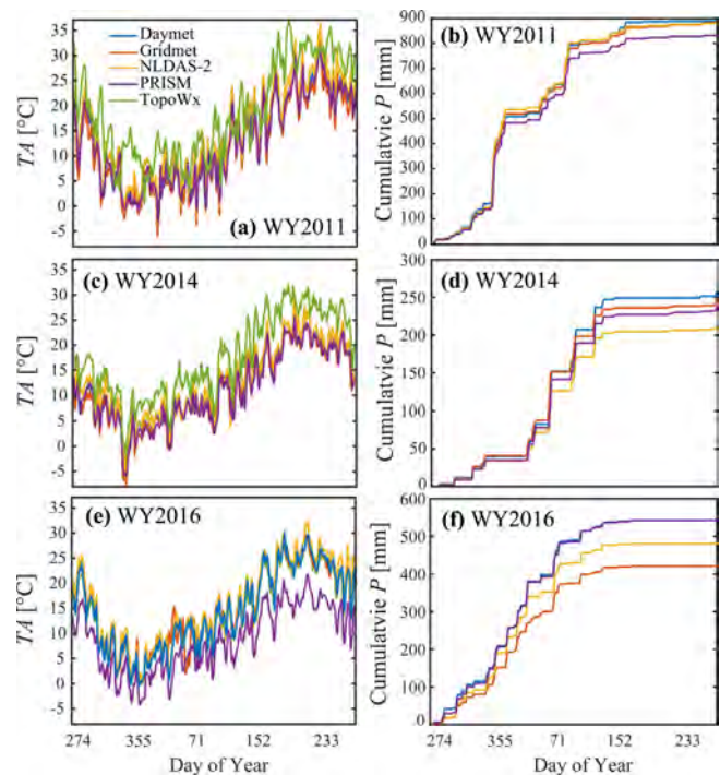
Figure 3. (a, c, e) Daily domain-averaged values of air temperature for five temperature datasets and (b, d, f) the cumulative sum of domain-averaged precipitation for each of the four gridded datasets in (a, b) WY2011, (c, d) WY2014, and (e, f) WY2016.
