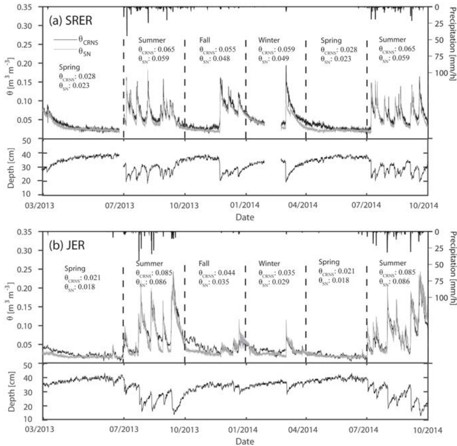
Figure 4. Comparison of the spatially averaged, hourly soil moisture ( \text{m}^3 \text{m}^{-3} ) from CRNS method ( \theta_{\text{CRNS}} , black lines) and distributed sensor network ( \theta_{\text{SN}} , gray lines) at (a) SRER and (b) JER, along with spatially averaged, hourly precipitation during 1 March 2013 to 30 September 2014. Vertical dashed lines indicate the seasonal definitions and their corresponding seasonally averaged \theta_{\text{CRNS}} and \theta_{\text{SN}} in \text{m}^3 \text{m}^{-3} . Also shown are the time-varying measurement depths ( z^* ).
